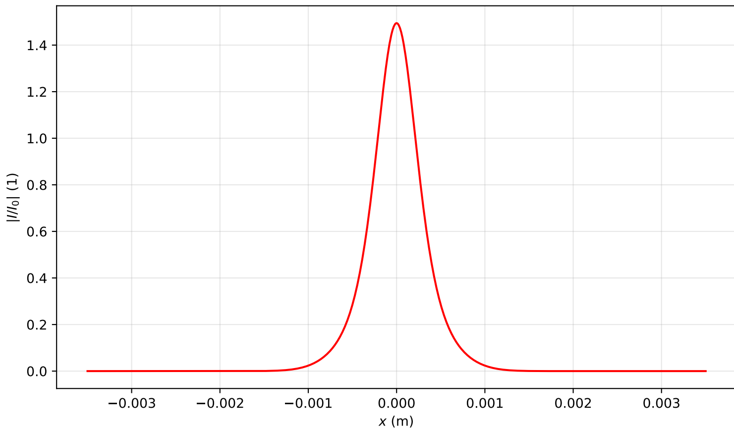
Intensity profile I(x, y = 0, z = 0.955)/I_0 , P_{in}=1.0P_{cr} , artificial time
